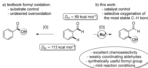
Scheme 1. Chemoselectivity in the C–H activation of benzaldehyde.
